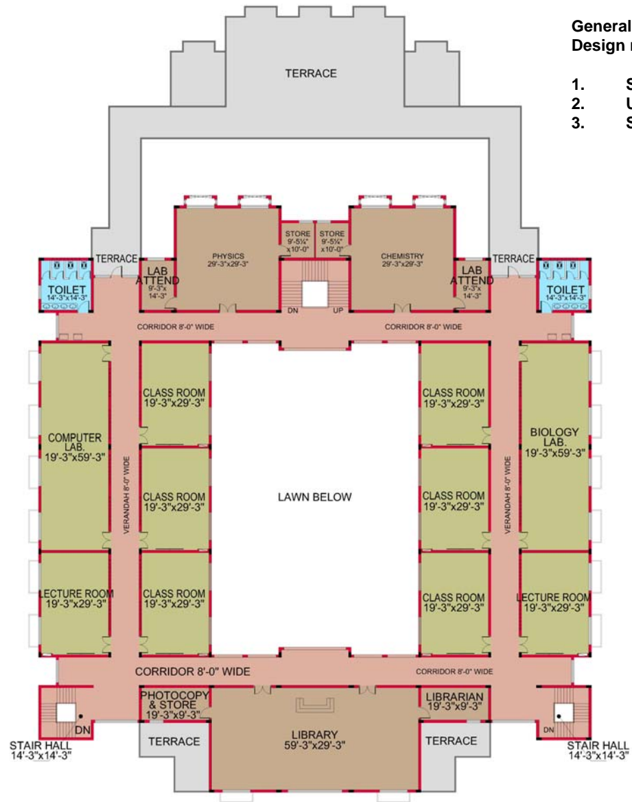
FIRST FLOOR PLAN COVERED AREA : 19,191 SFT
